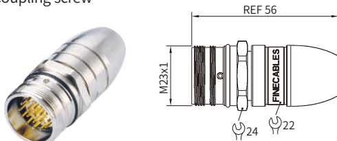
Coupling screw
