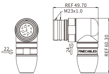
Coupling screw
