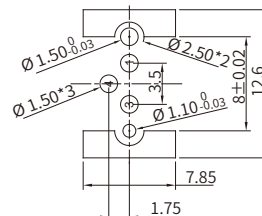
03 Pins Female
