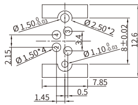
04 Pins Male
