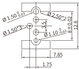
03 Pins Male
