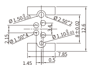
04 Pins Female
